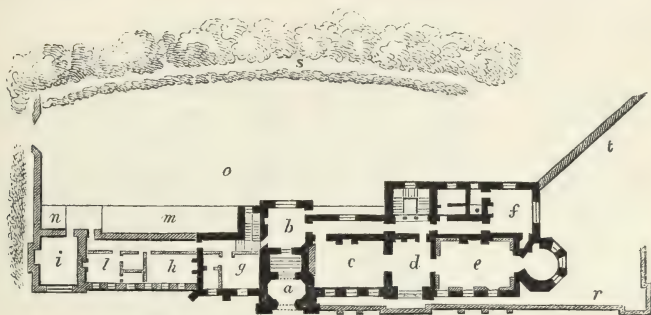
[Fig. 106. Example of a plan for an extended front on the steep side of a hill.]
